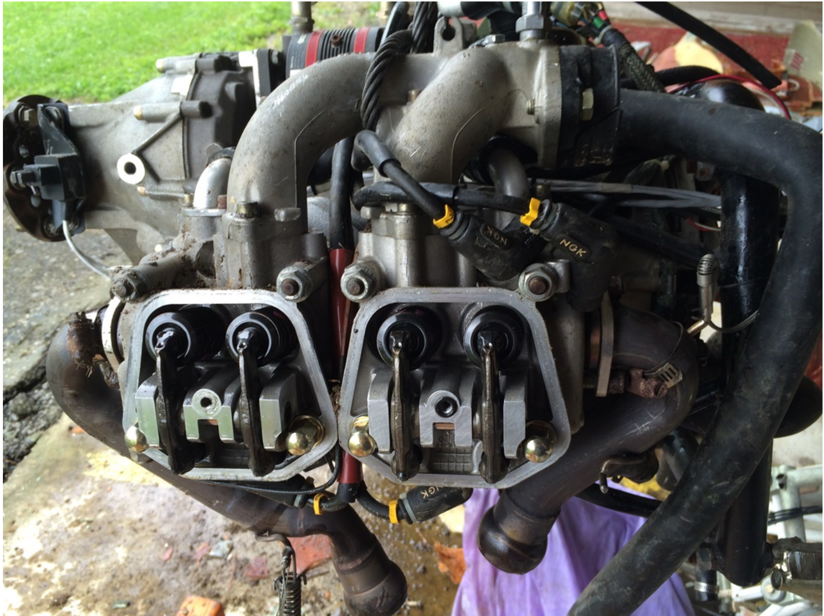
Photo 3 - Engine
