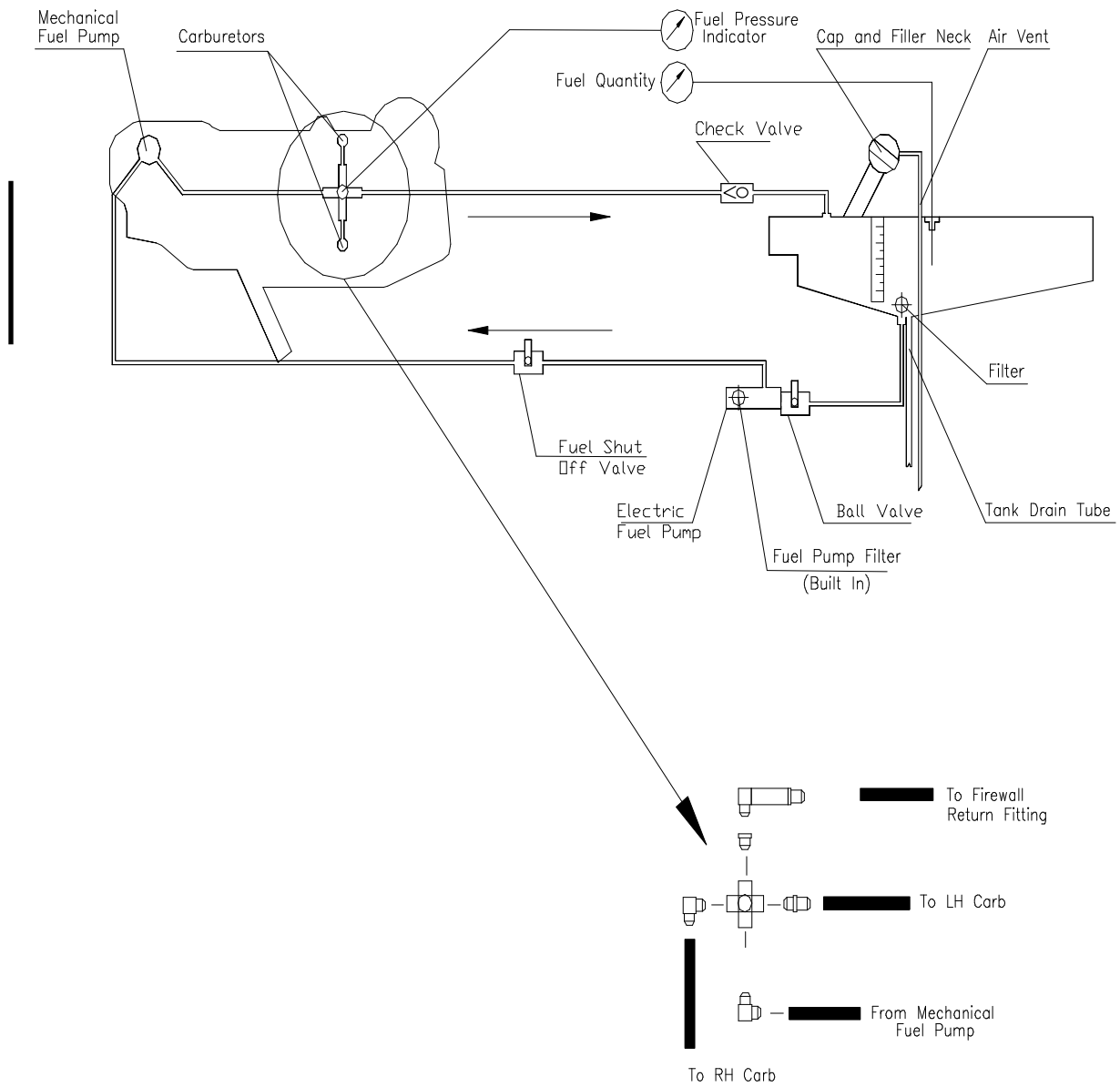
Figure 1: Fuel System (S/N 10002 through 10092)
