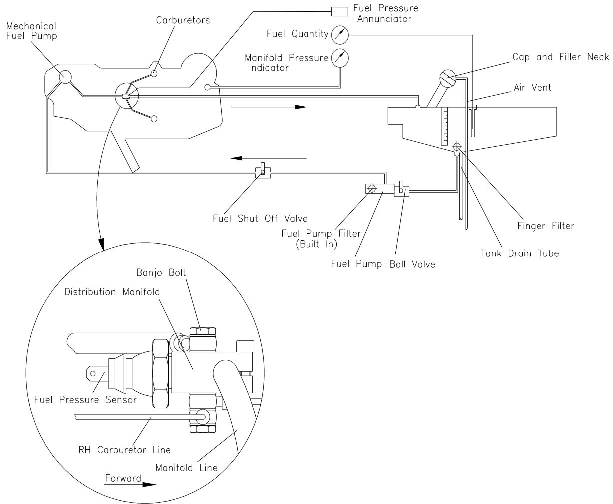
Figure 2: Fuel System (S/N 10093 and subsequent and aircraft serial number 10002 to 10092 with service bulletin DA20-73-01 or DA20-73-03 incorporated)
