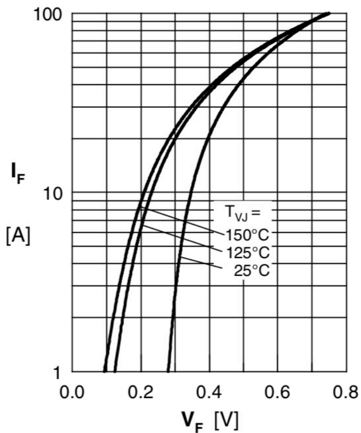
Fig. 1 Maximum forward voltage drop characteristics
