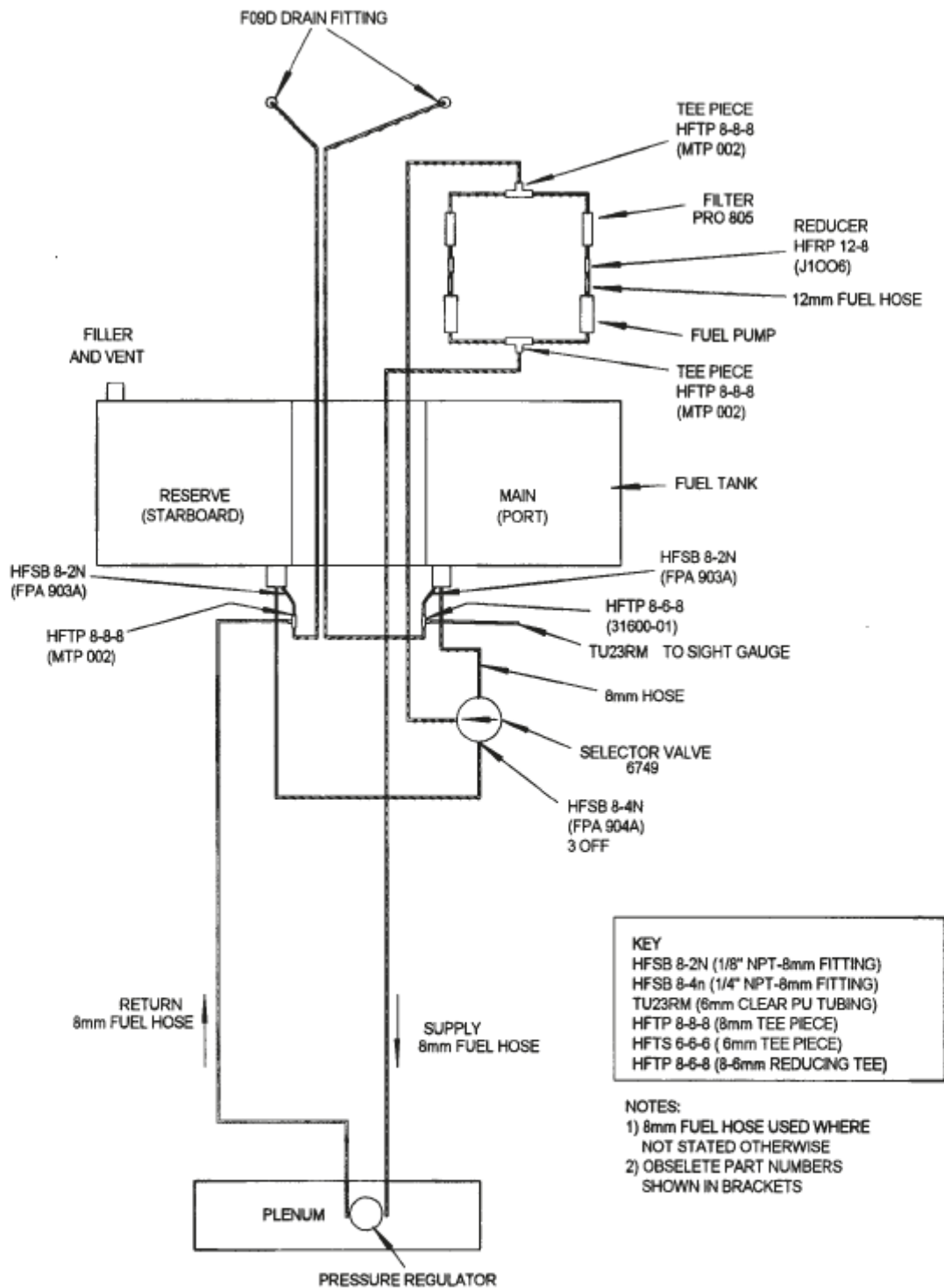
ROTAX 914 FUEL SYSTEM WITH WATER DRAINS (PARALLEL PUMP SYSTEM SHOWN)
