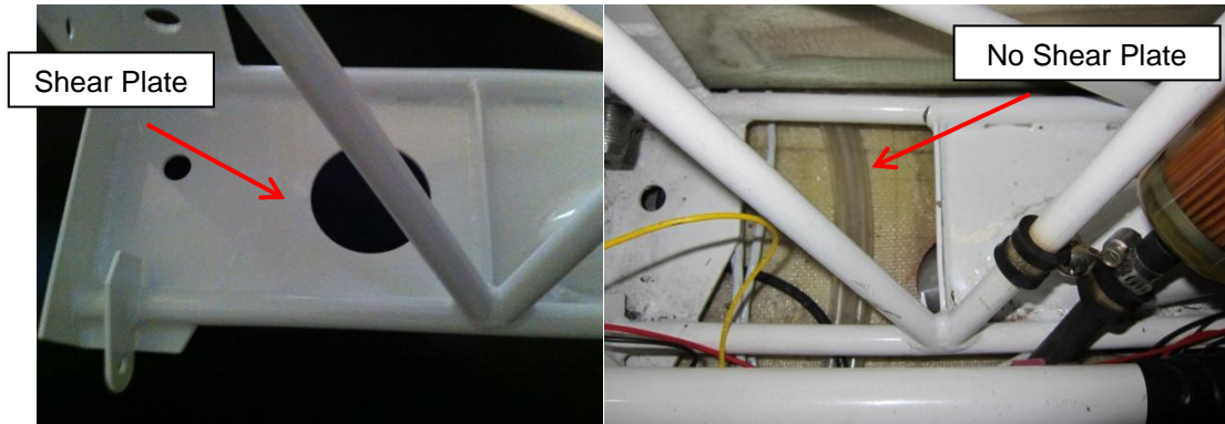
Figure 5, New Spar Box Left Side vs Old Spar Box
