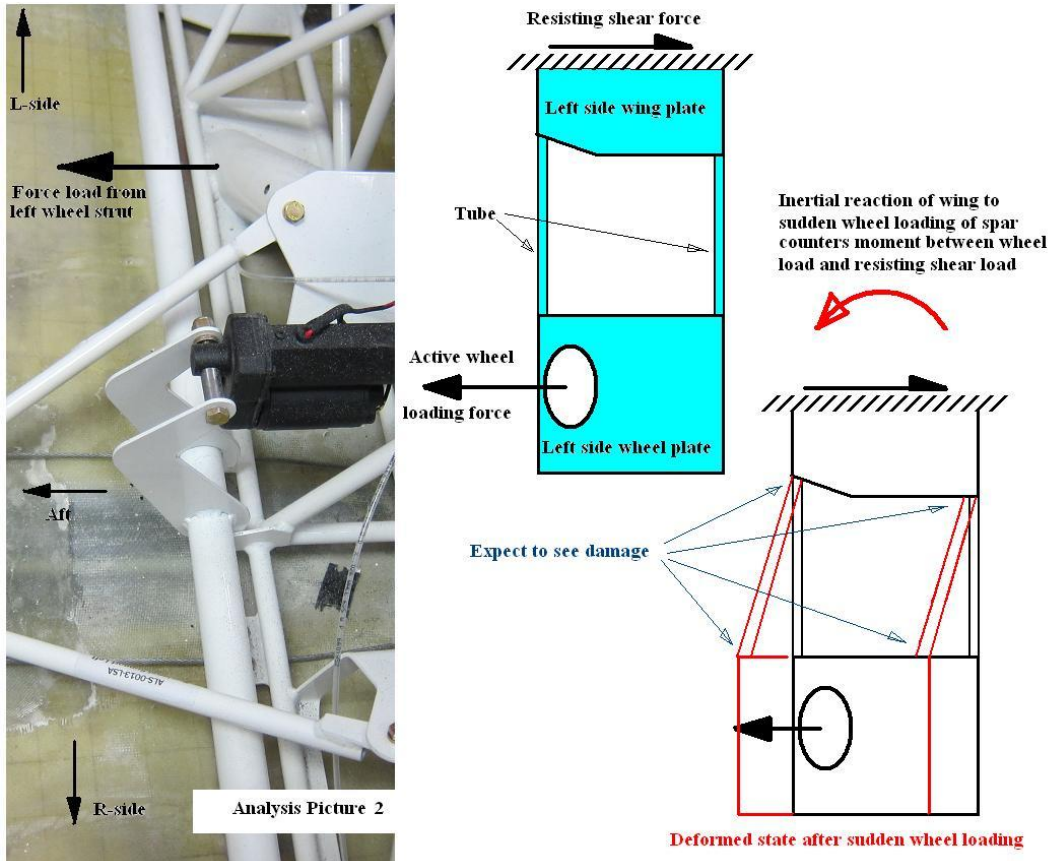
Figure 3: Analysis of Spar Box Structure, Picture 2
