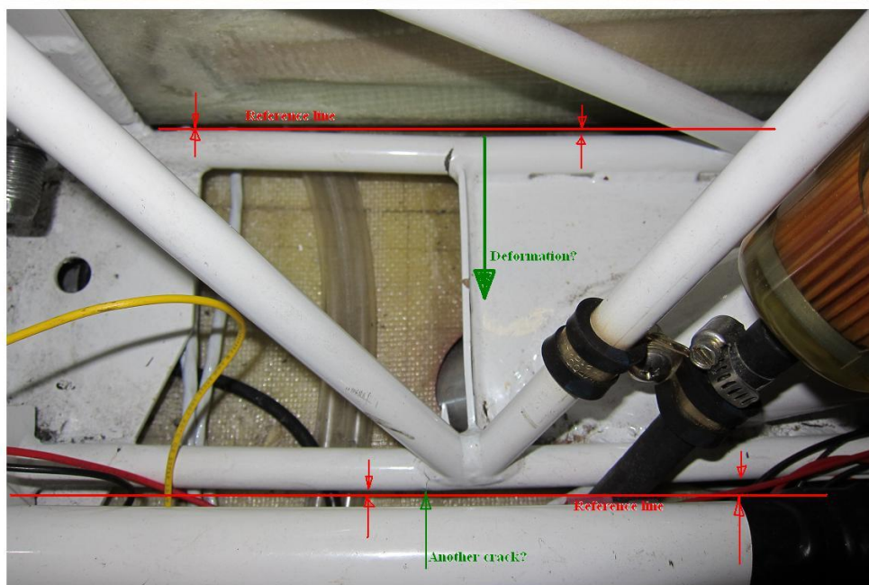
Figure 4: My Cracked Spar Box with Analysis
