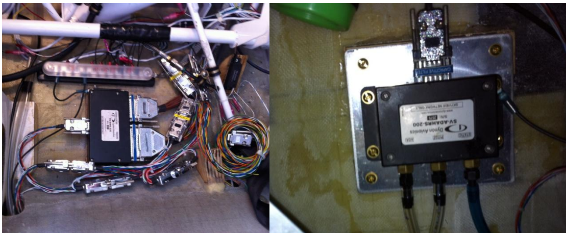
Figure 8: Engine Monitoring Computer (left) and ADAHRS (right).
