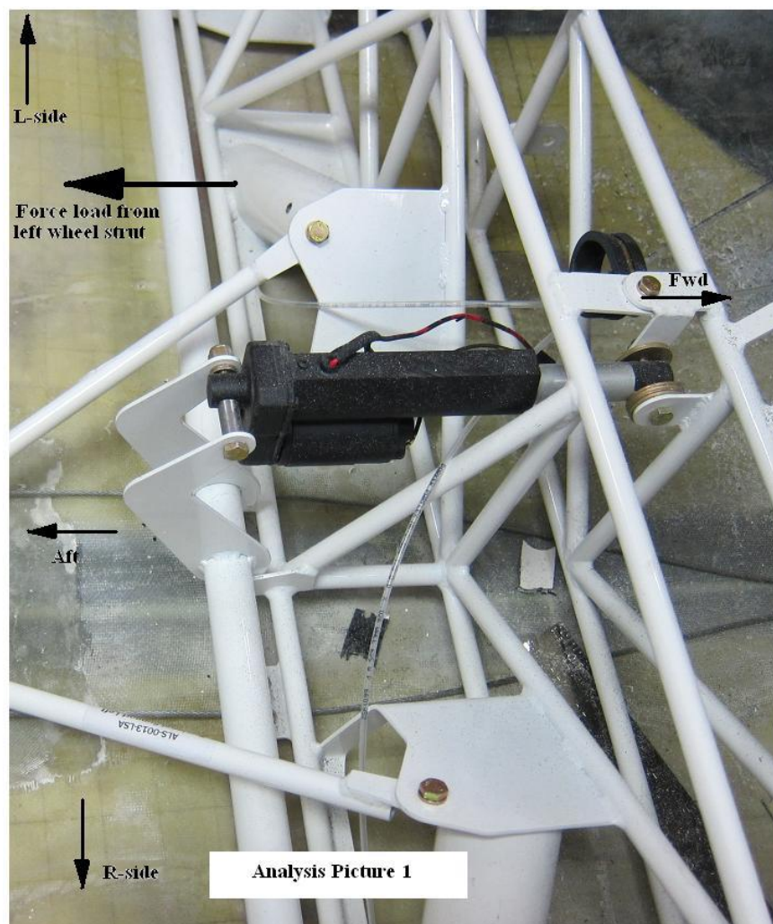
Figure 2: Analysis of Spar Box, Picture 1
