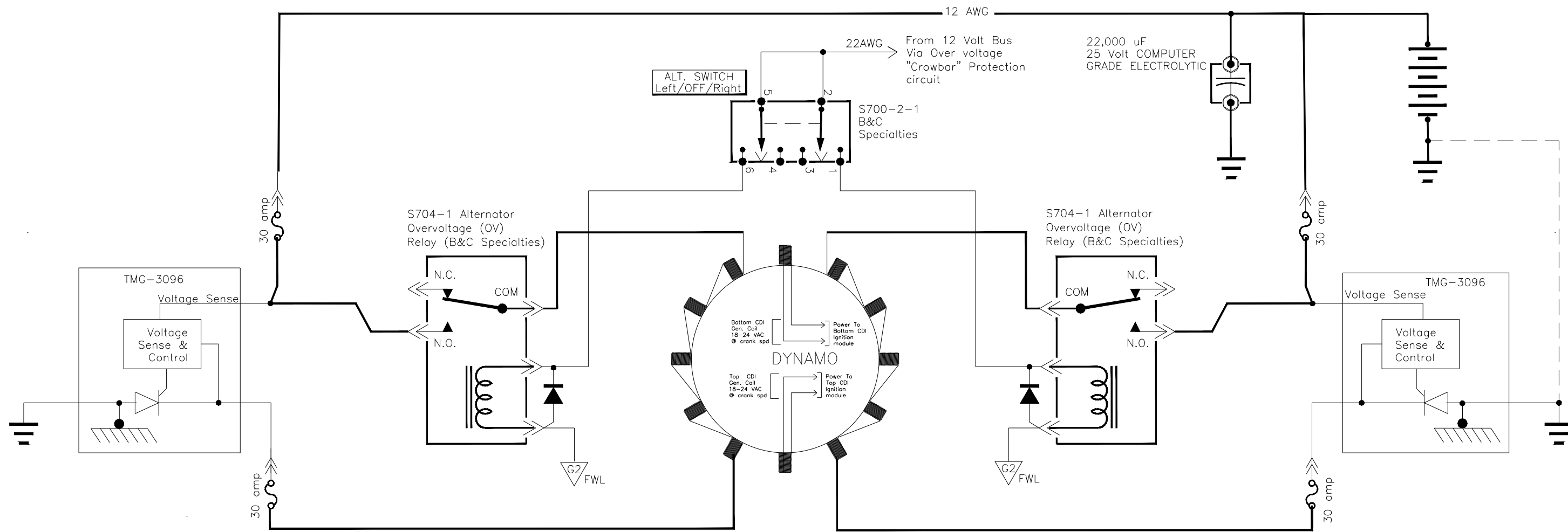
Equivalent Alternator Circuit
