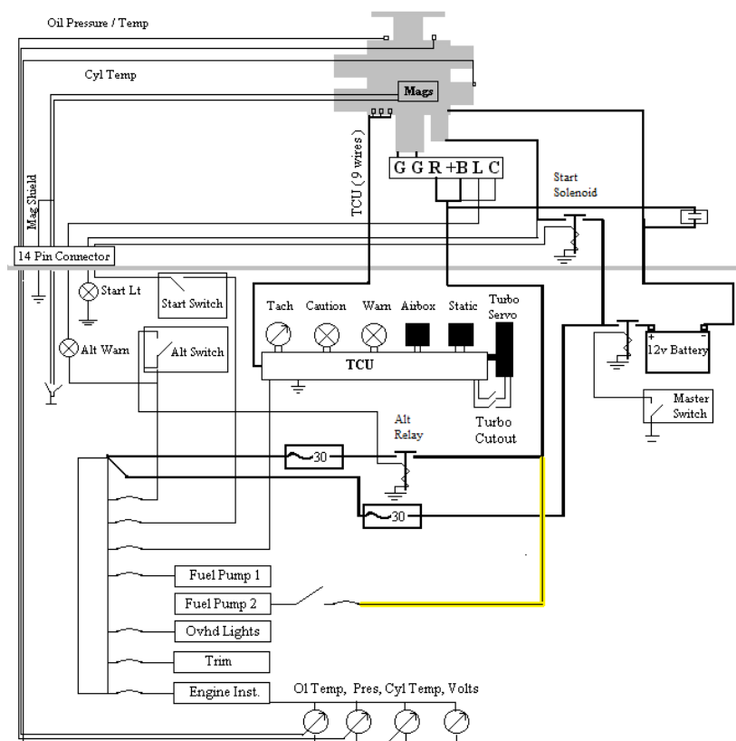
Rotax Power Distribution Using Relay for Alternator Control
