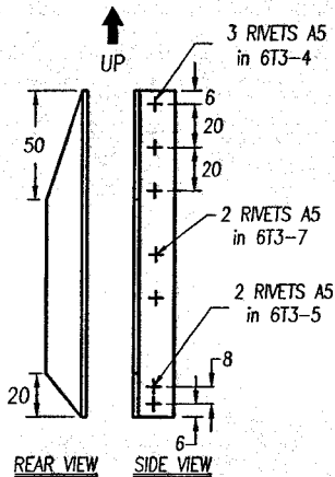
6 ELEVATOR HORN DOUBLER EXT 6061-T6 3/4"x3/4"x.093" (1 REQ'D) length = 160
