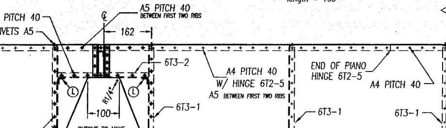
6 ELEVATOR HORN DOUBLER EXT 6061-T6 3/4"x3/4"x.093" (1 REQ'D) length = 160
