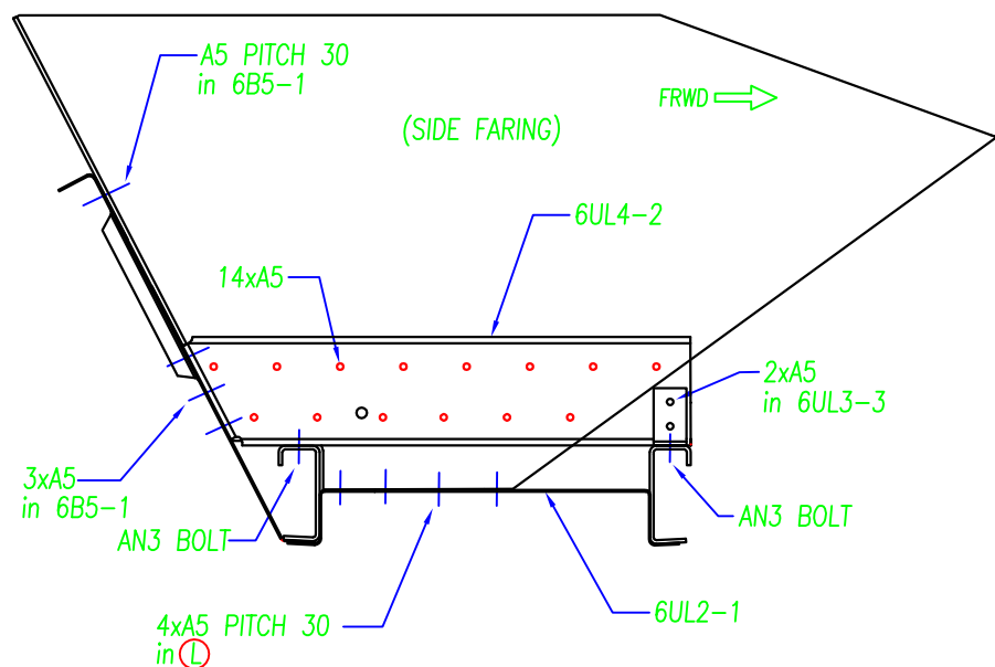
SIDE VIEW
