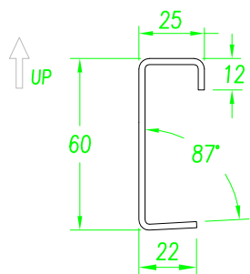
SIDE FAIRING
