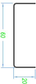
2 GUARD 6061-T6 t=.025" L=300 (1 REQ'D)
