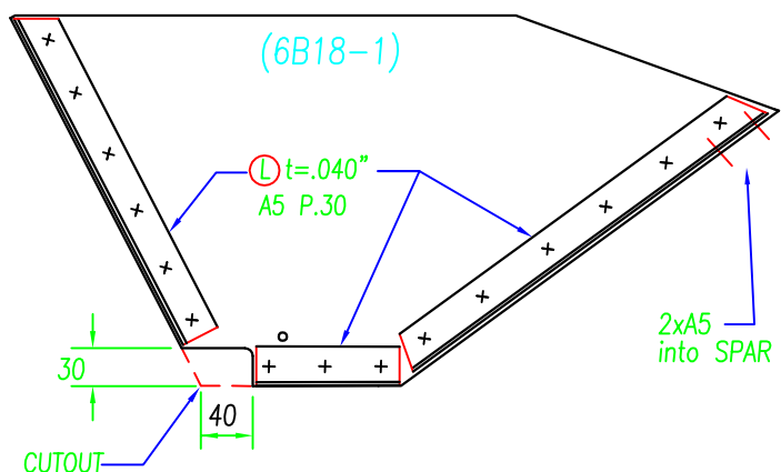
SIDE FAIRING
