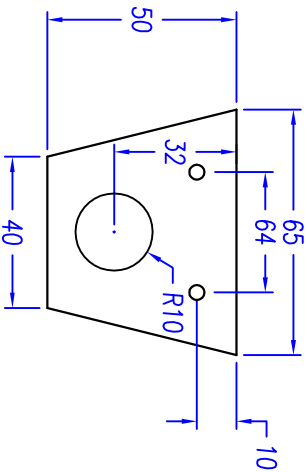
2 TAIL DRAG BOTTLE HOLDER
