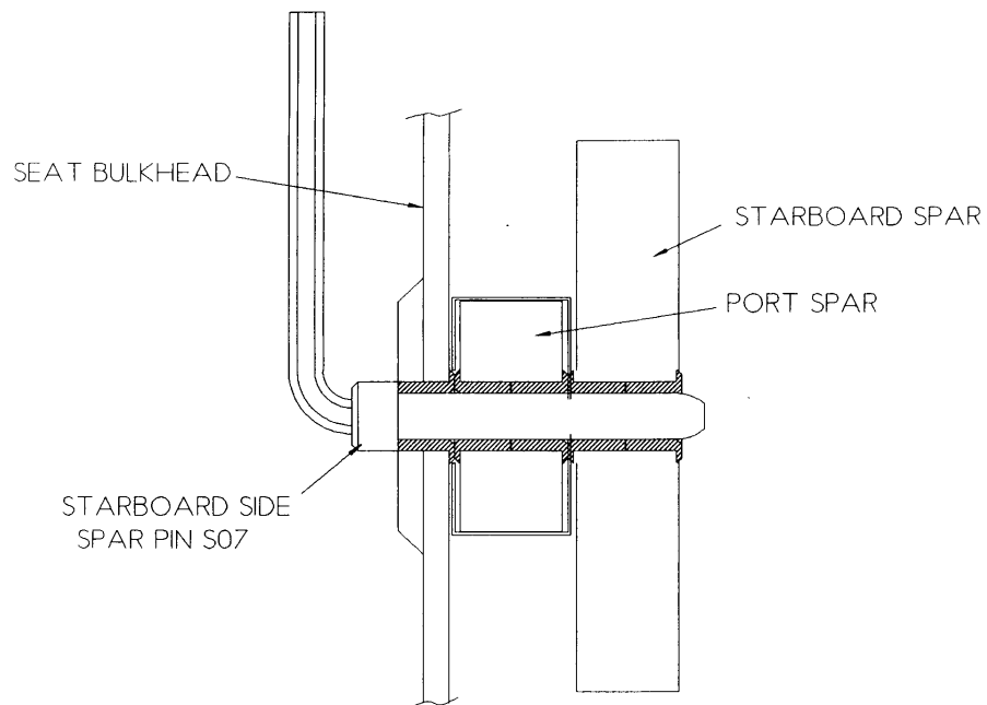
Fig 2. Section through starboard side spar pin area.
