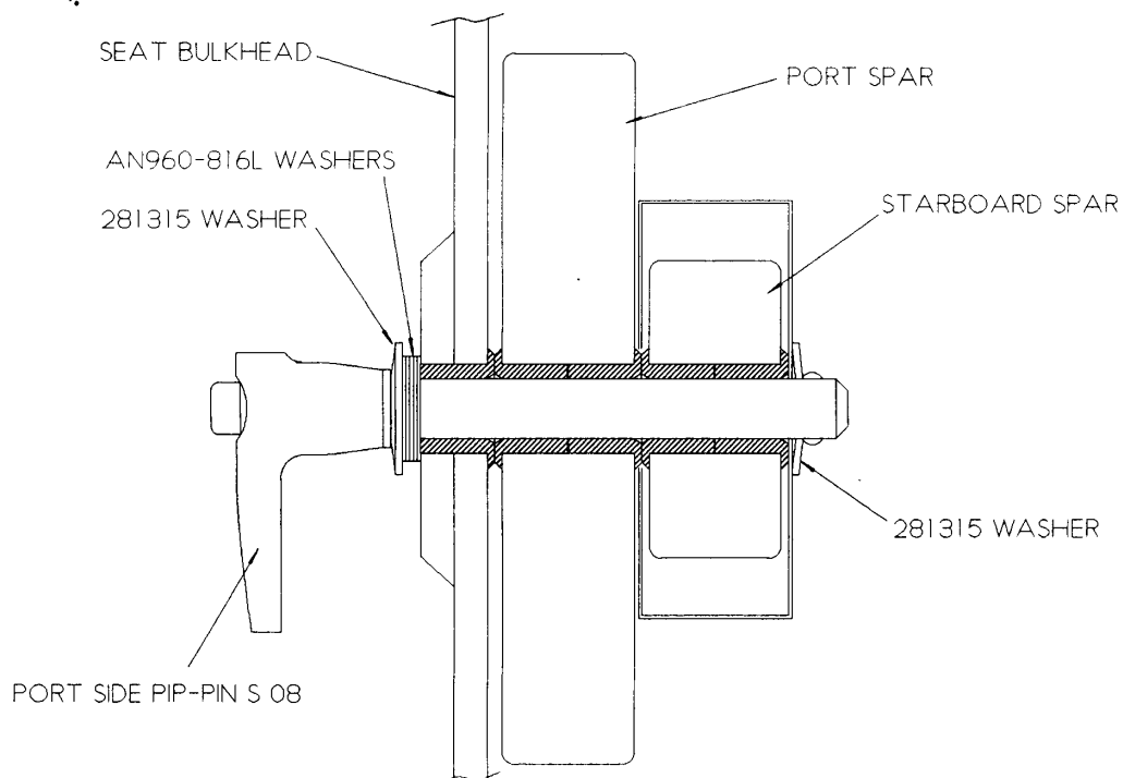
Fig 1. Section through port side spar pin bush area.
