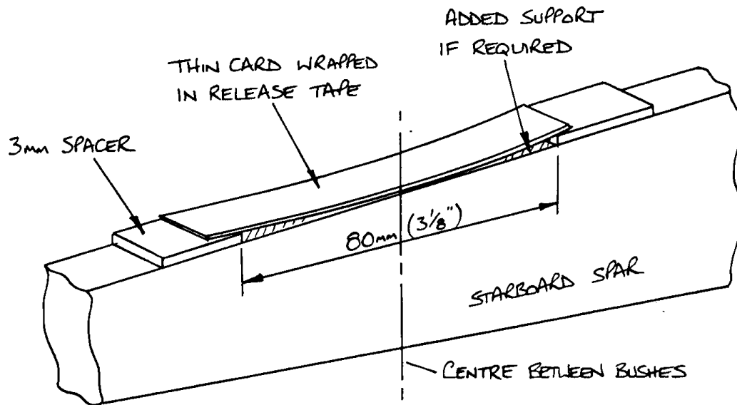
Fig 12. Former position on spar.
