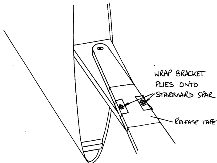
Fig 14. Brackets wrapped around starboard spar.
