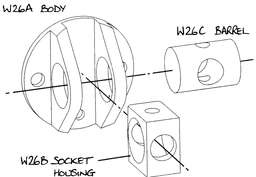
Fig 6. Exploded view of W26 wing rear pin socket assembly
