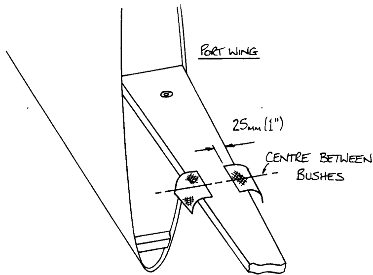
Fig 13. Bracket plies in position on port spar.
