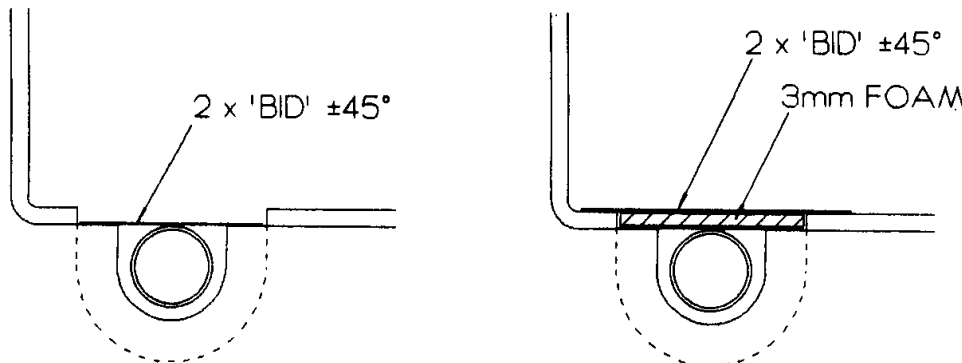
Fig 11. Section through tunnel detailing layup sequence.
