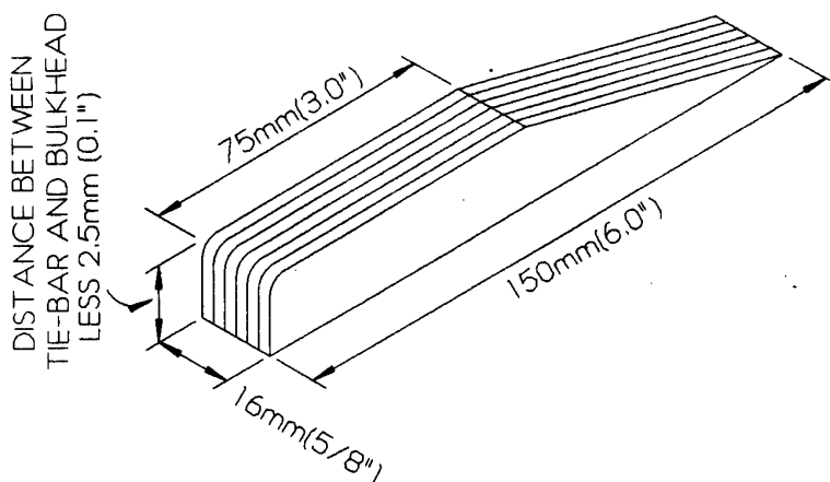
Fig 9. Plywood block for gusset plates.
