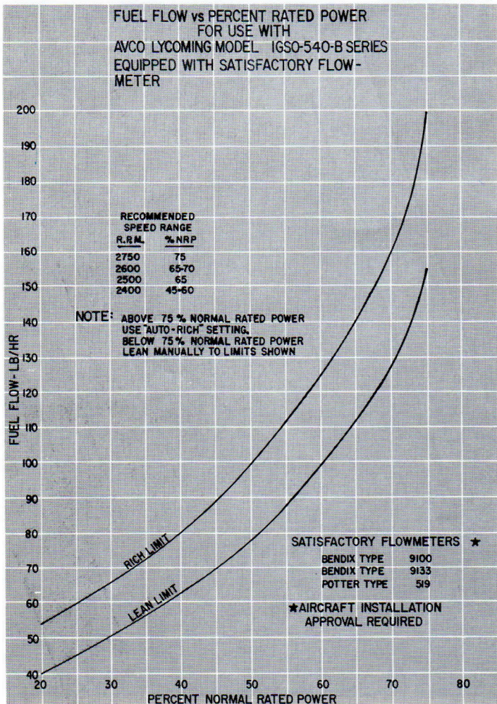
Figure 3-5. Fuel Flow vs Percent Rated Power - IGSO-540-B Series
