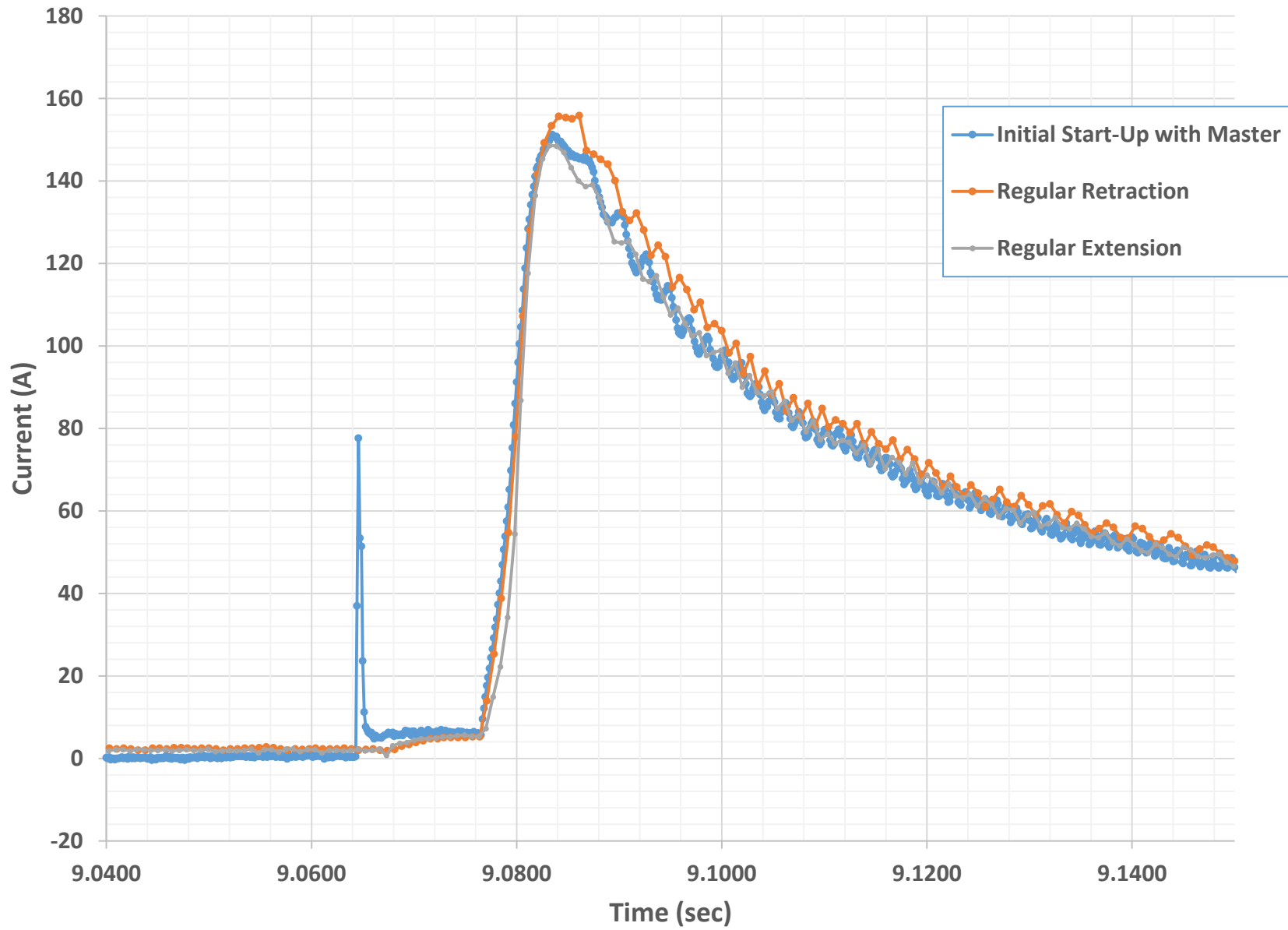
Legacy Hydraulic Pump Start-up Current
